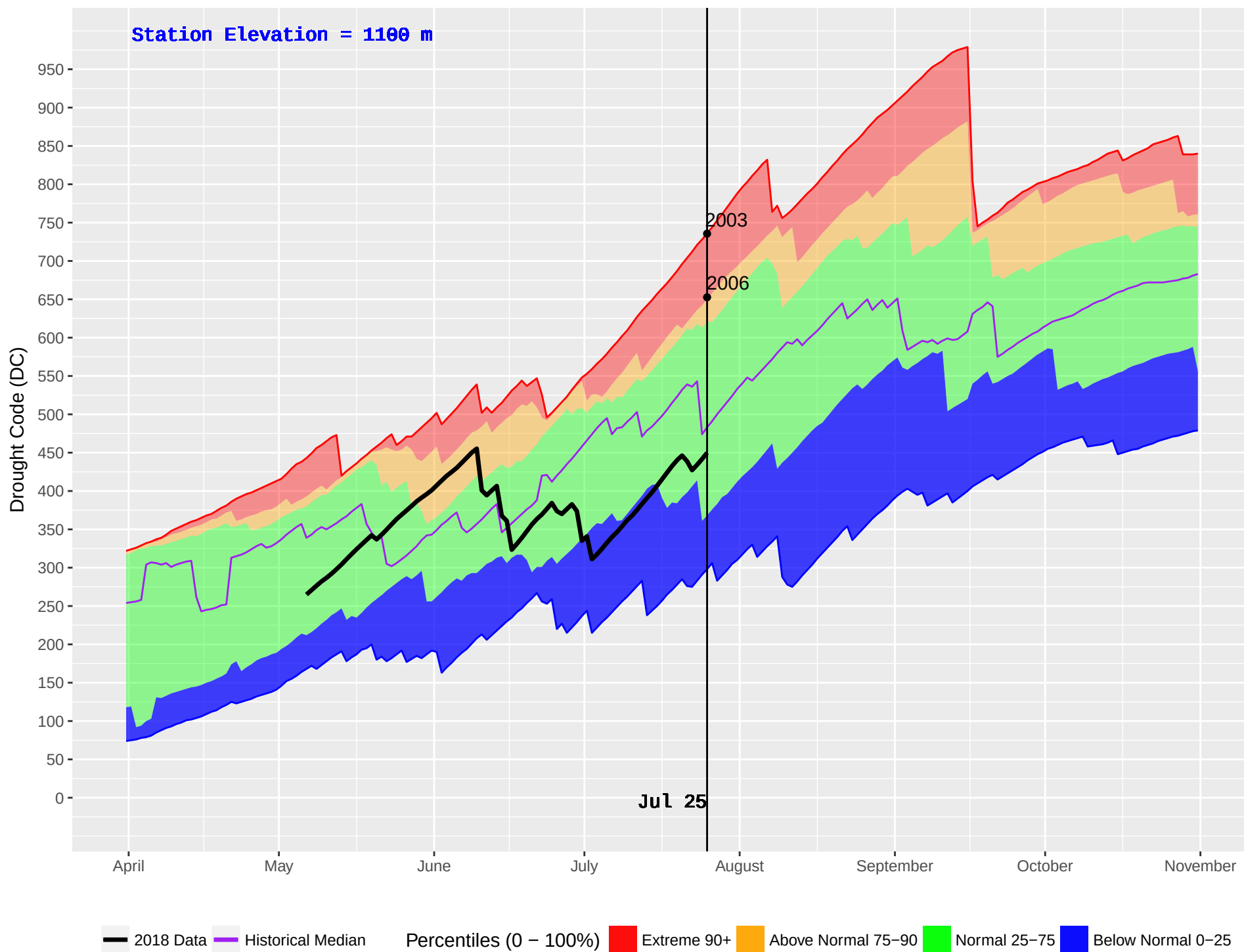
CHURN CREEK (832) : Historical (2003–2016) and Current (2018) Noon Drought Code (DC)
