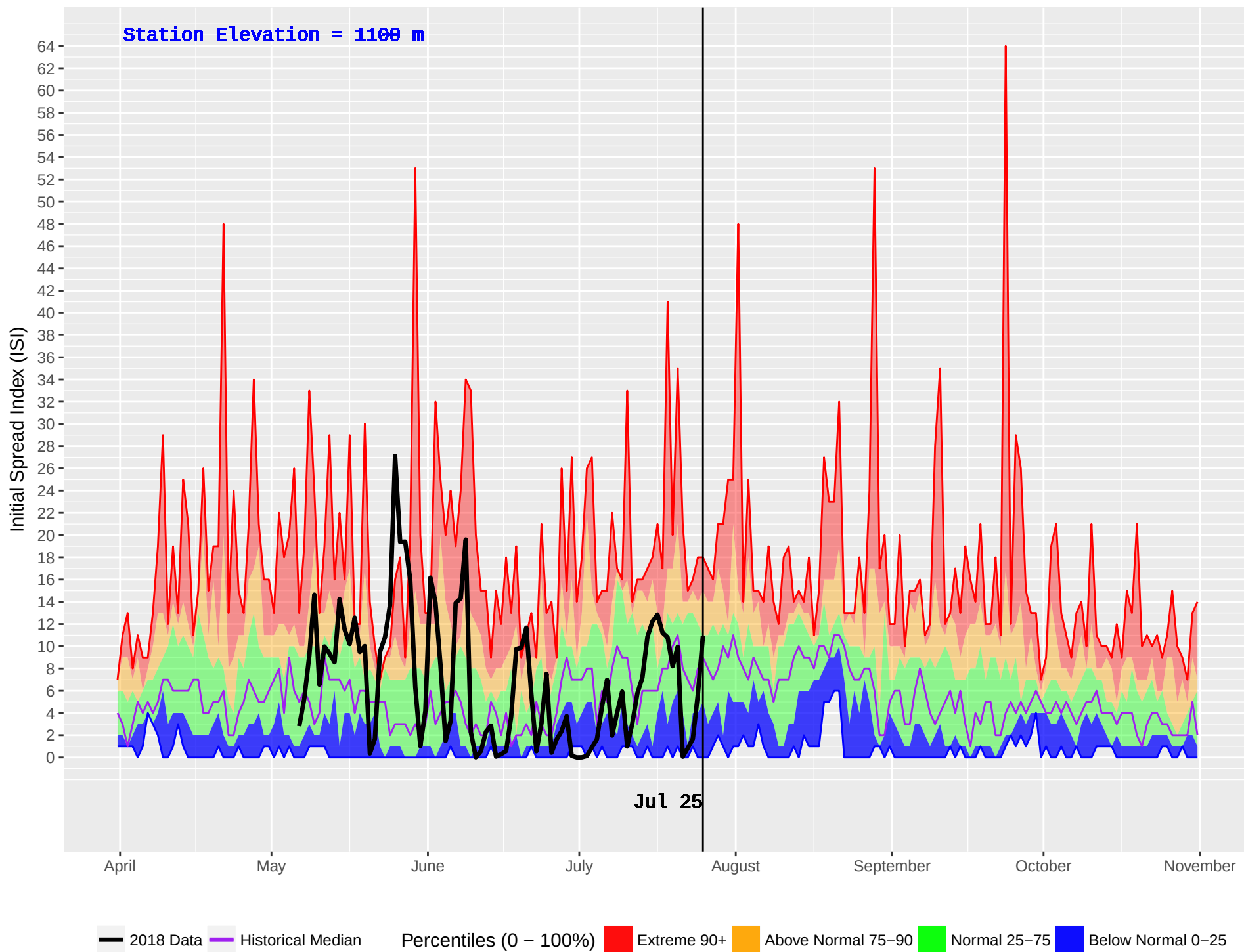
CHURN CREEK (832) : Historical (2003–2016) and Current (2018) Noon Initial Spread Index (ISI)
