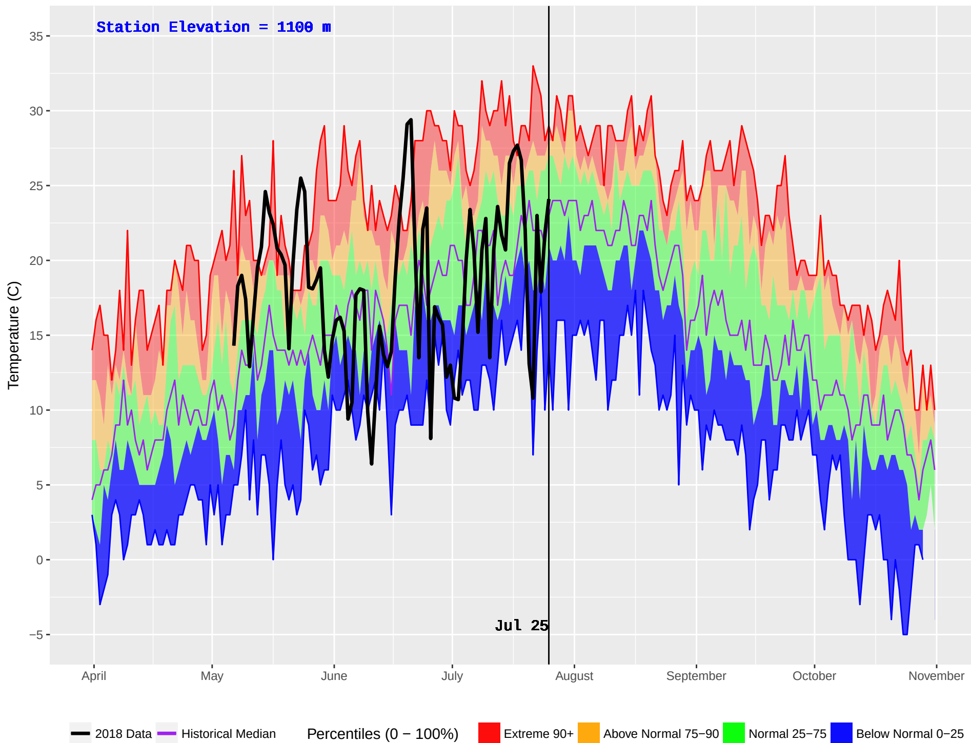
CHURN CREEK (832) : Historical (2003–2016) and Current (2018) Noon Temperature
