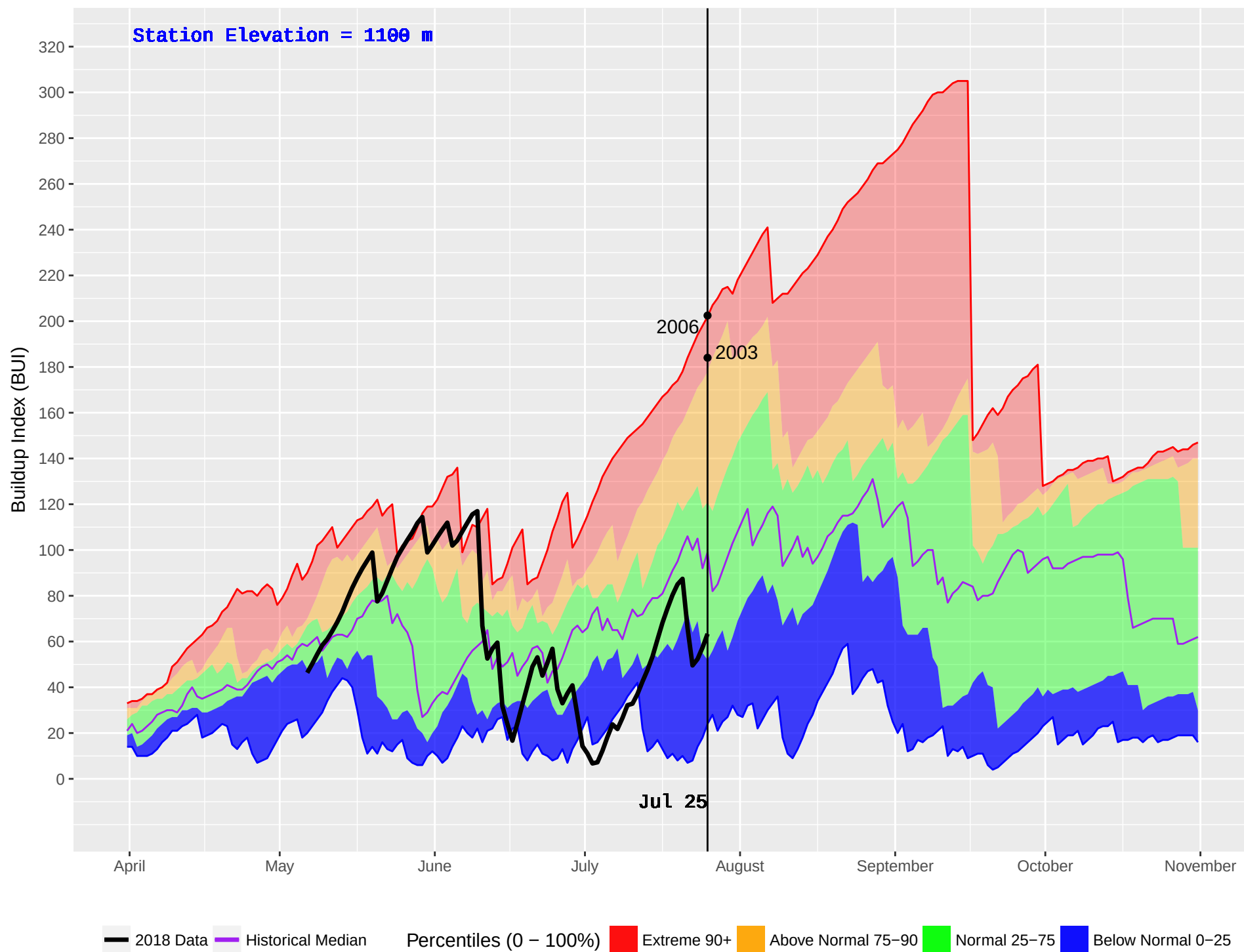
CHURN CREEK (832) : Historical (2003–2016) and Current (2018) Noon Buildup Index (BUI)
