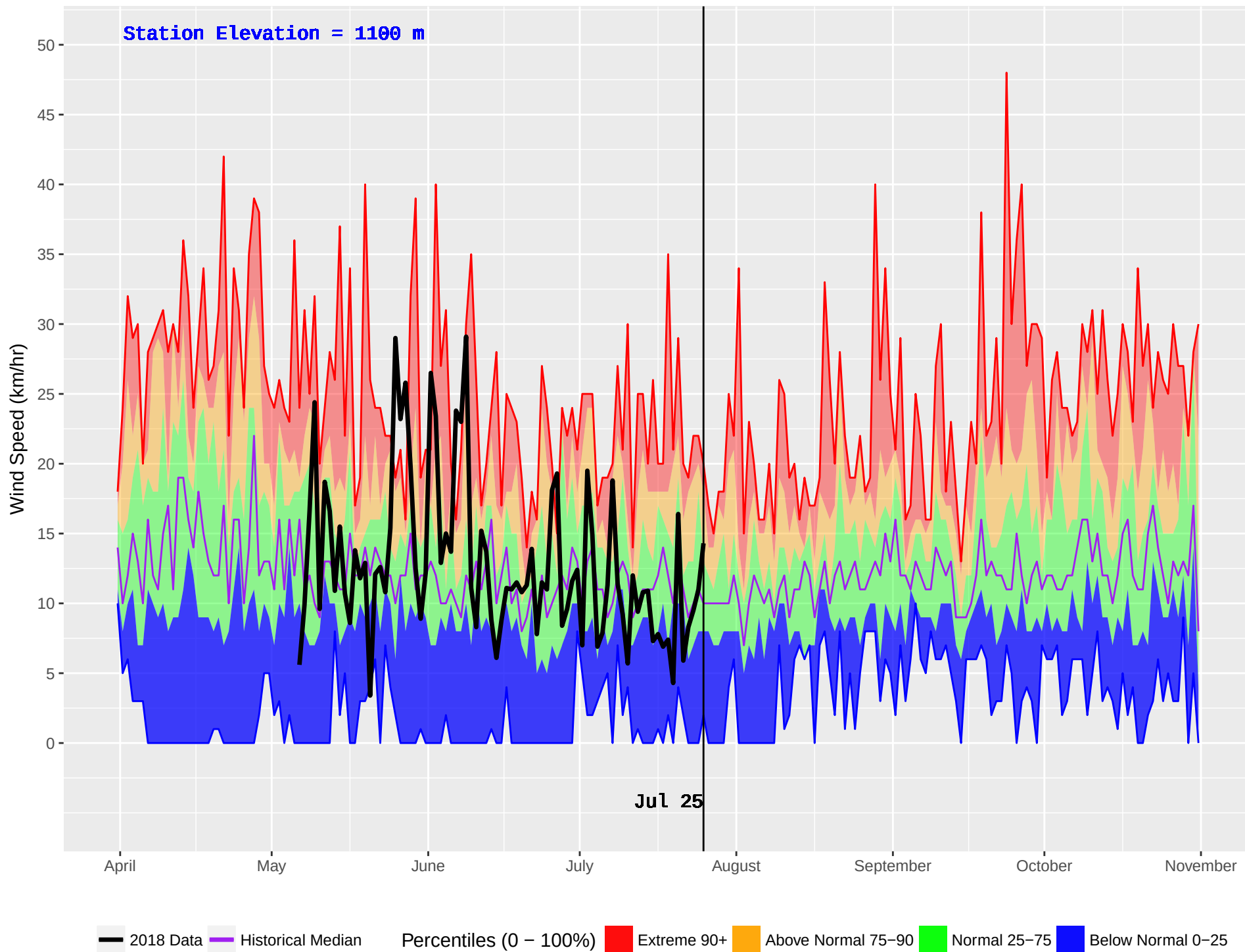
CHURN CREEK (832) : Historical (2003–2016) and Current (2018) Noon Wind Speed
